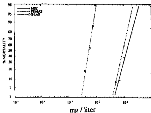
Fig. 2. Concentration-mortality lines obtained in bioassays of chlorpyrifos with the susceptible reference strain S-LAB and the 2 resistant strains MSE and PRAIAS. The bioassays were done: (A) in absence of synergists, (B) in presence of DEF, and (C) in presence of PB.
